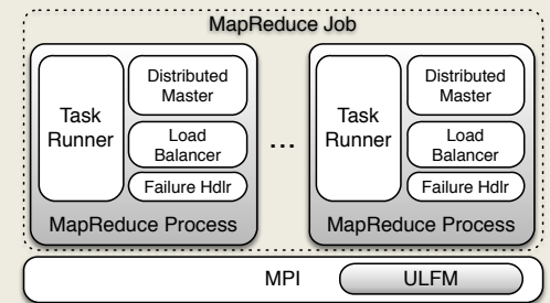
MapReduce
