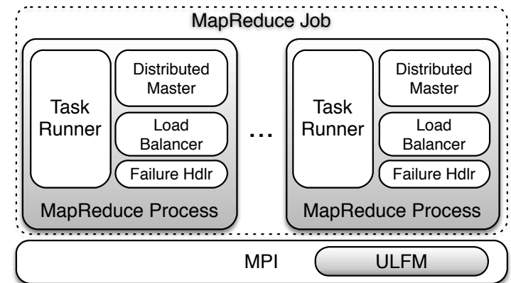
Figure 2: The architecture of FT-MRMPI.
