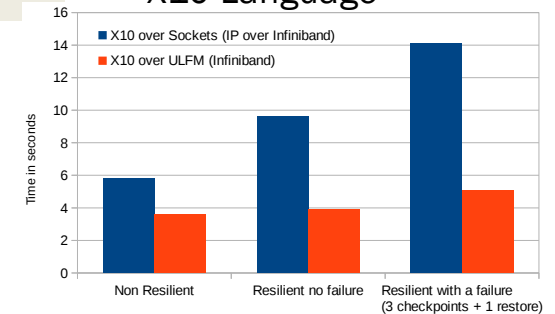
X10 Language
