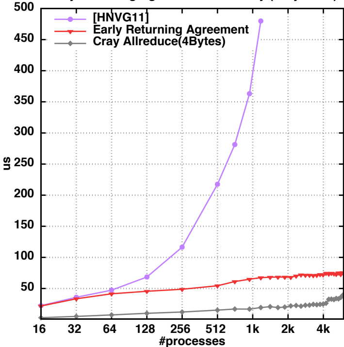
Early Returning Agreement Scalability (Cray XC30)
