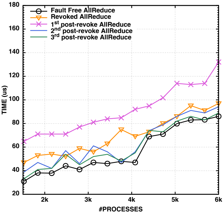
Revoke Time and Perturbation in AllReduce (4Bytes)
